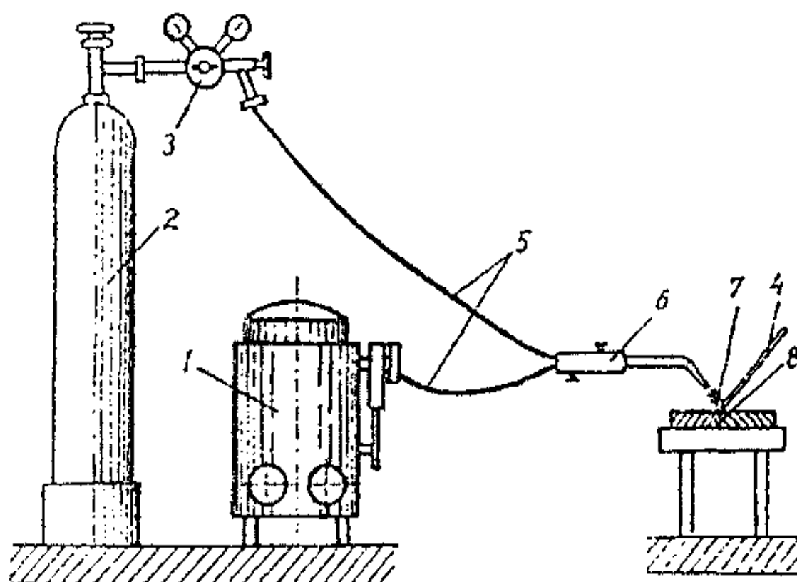
5.34-rasm. Gaz alangasida payvandlash: 1 – gazogenerator; 2 – kislorodli ballon; 3 – reduktor; 4 – qo'shimcha sim; 5 – shlanglar; 6 – gaz gorelkasi; 7 – alanga; 8 – payvand chok.
