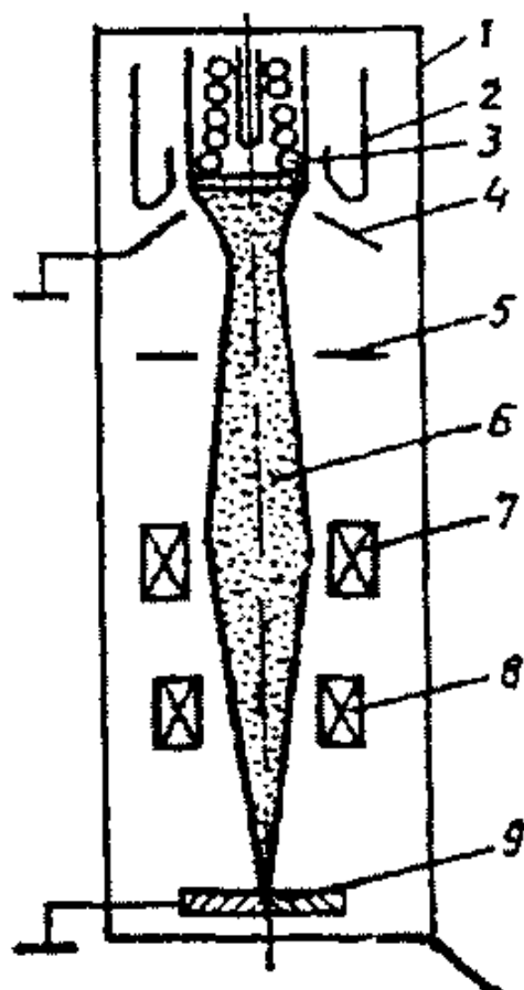
5.35-rasm. Elektron-nur yordamida payvandlash: 1 – vakuum kamerasi; 2 – shakllantiruvchi elektrod; 3 – volfram katod; 4 – anod; 5 – diafragma; 6 – elektron-nur; 7 – fokuslovchi magnit linzalar; 8 – ogʻdiruvchi sistema; 9 – payvandlanadigan detal.
