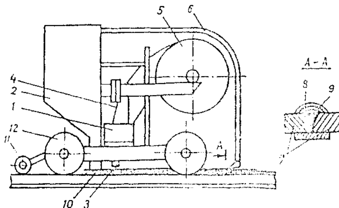
5.32-rasm. Flyus qatlam ostida avtomatik payvandlash:
