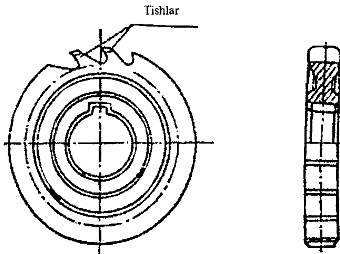
5.47-rasm. Paz ochadigan disk freza.
