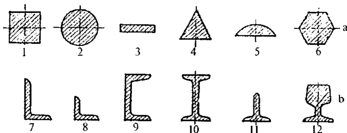
5.12-rasm. Navaviy prokat profillari: a — oddiy;
