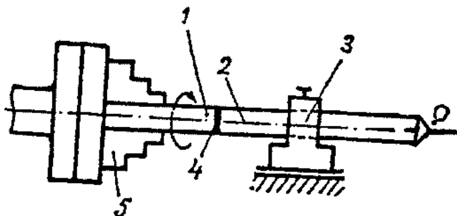
5.38-rasm. Ishqalanish vositasida payvandlash:
