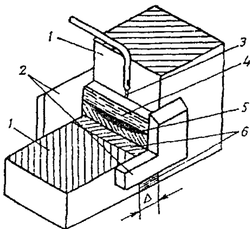
5.33-rasm. Elektr-shlak usulida payvandlash:
