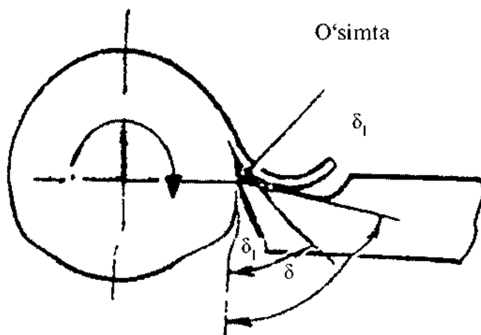
5.40-rasm. O'simtaning o'tkirlanish burchagiga ta'siri.
