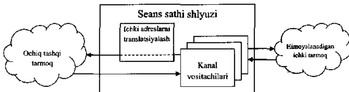
8.8-rasm. Seans sathi shlyuzining ishlash sxemasi.
