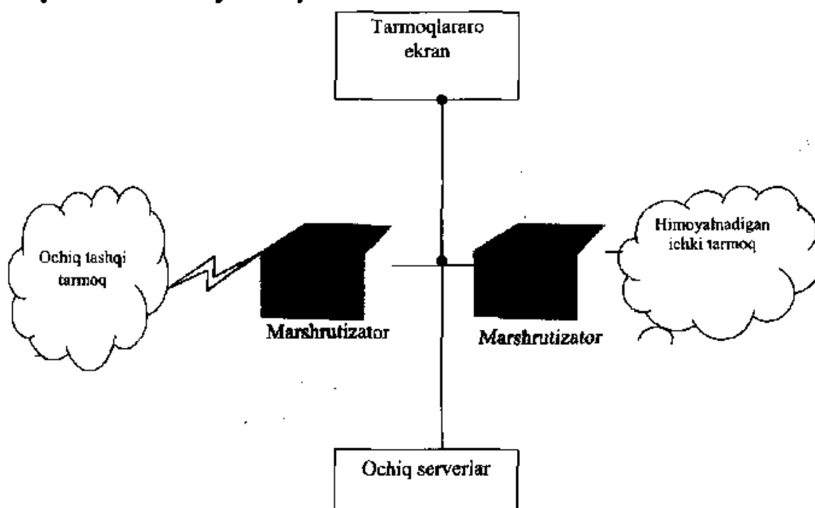
8.11- rasm. Bitta tarmoq interfeysli firewall yordamida lokal tarmoqni himoyalash.
