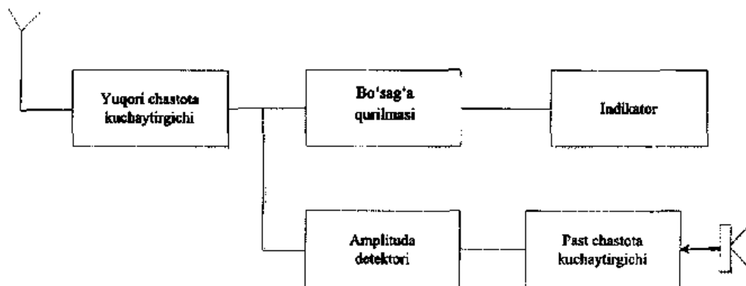
10.4-rasm. Elektromagnit nurlanish indikatorining sxemasi.
