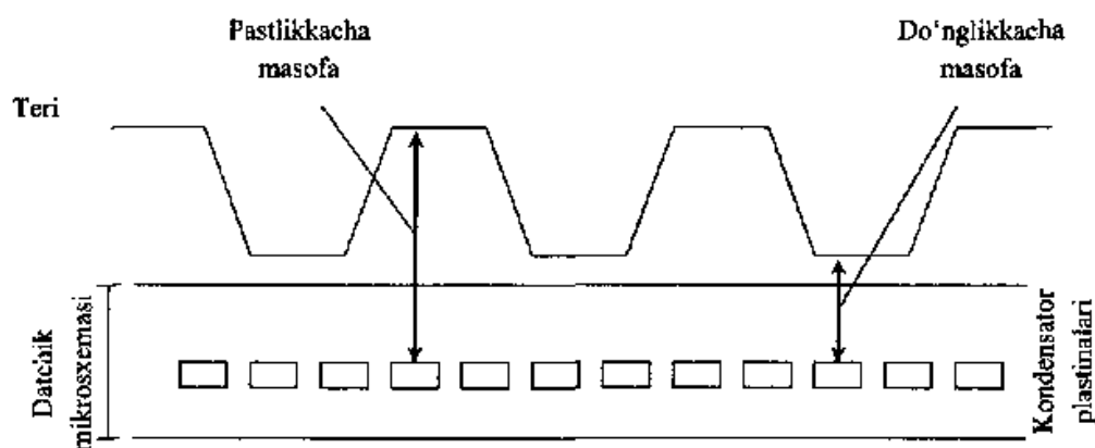
6.6-rasm. Sensor ishlashining prinsipi.
