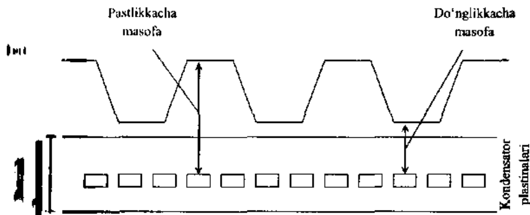
6.6-rasm. Sensor ishlashining prinsipi.
