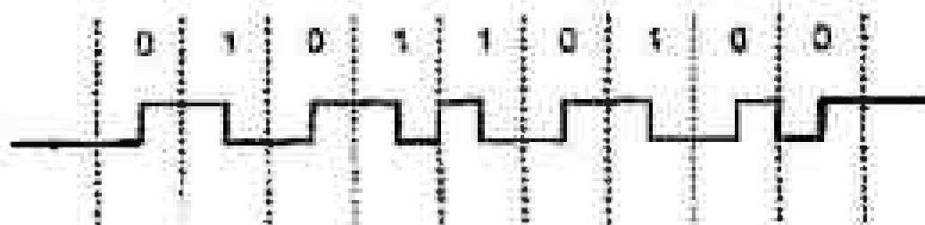
5.17-rasm. Manchester kodl.
