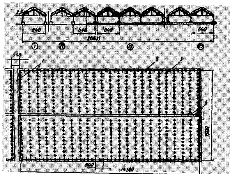
13-rasm. Qishki blokli issiqxonaning old tomoni ko‘rinishi va rejasi (mm):
