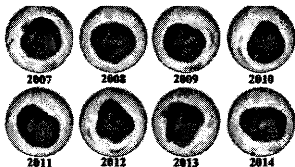
8.4-rasm. Ozon qatlamining hozirgi holati (Levashov, 2015)
