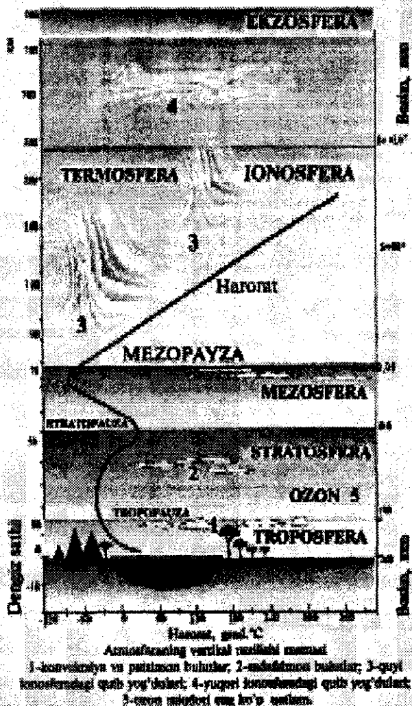
8.1-rasm. Atmosferaning vertikal tuzilishi (R.Ramade, 1998 y).
